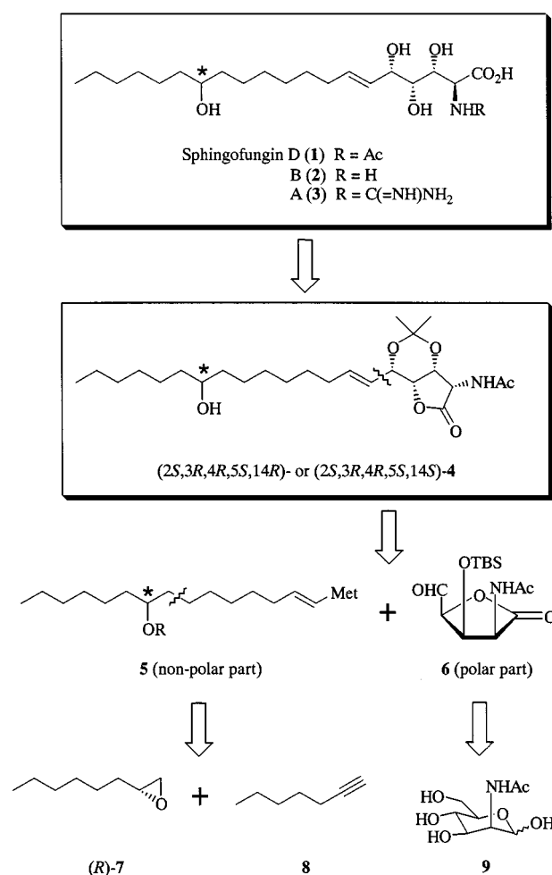
Scheme 1. Structures of sphingofungins and their retrosynthetic analysis
