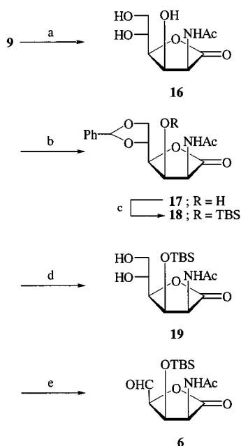
Scheme 3. Synthesis of the polar building block 6 ; reagents: (a) Br 2 , H 2 O (41%); (b) PhCH(OMe) 2 , HBF 4 ·OEt 2 , DMF (98%); (c) TBSCl, 2,6-lutidine, CH 2 Cl 2 (65%); (d) Pd(OH) 2 , cyclohexene, EtOH (85%); (e) NaIO 4 , H 2 O, CH 2 Cl 2 (crude 95%)
