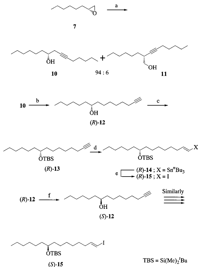
Scheme 2. Synthesis of the nonpolar building block 15 ; reagents: (a) 1) 1-heptyne ( 8 ), n BuLi, BF 3 ·OEt 2 , THF; 2) ( R )- 7 (80%); (b) Li, t BuOK, H 2 N[CH 2 ] 3 NH 2 (88%); (c) TBSCl, imidazole, DMF (quant.); (d) ( n Bu) 3 SnH, AIBN (92%); (e) I 2 , Et 2 O (95%); (f) 1) EtO 2 CN=NCO 2 Et, Ph 3 P, PhCO 2 H; 2) K 2 CO 3 , MeOH (80%)
