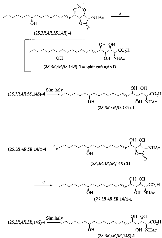
Scheme 5. Synthesis of sphingofungin D and its three stereoisomers; reagents: (a) 1) AcOH, THF, \text{H}_2\text{O} ; 2) MeOH, \text{H}_2\text{O} (59%); (b) AcOH, THF, \text{H}_2\text{O} (95%); (c) LiOH, THF, \text{H}_2\text{O} (78%)
