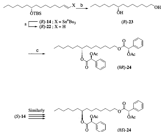
Scheme 6. Synthesis of optically active tetradecane-1,8-diol ( 23 ); reagents: (a) silica gel, n -hexane (quant.); (b) 1) \text{O}_3 , MeOH then \text{NaBH}_4 , EtOH, \text{H}_2\text{O} ; 2) HF aq., MeCN (85%); (c) ( S )-(+)- O -acetylmandelic acid, DCC, DMAP, \text{CH}_2\text{Cl}_2 (89%)
