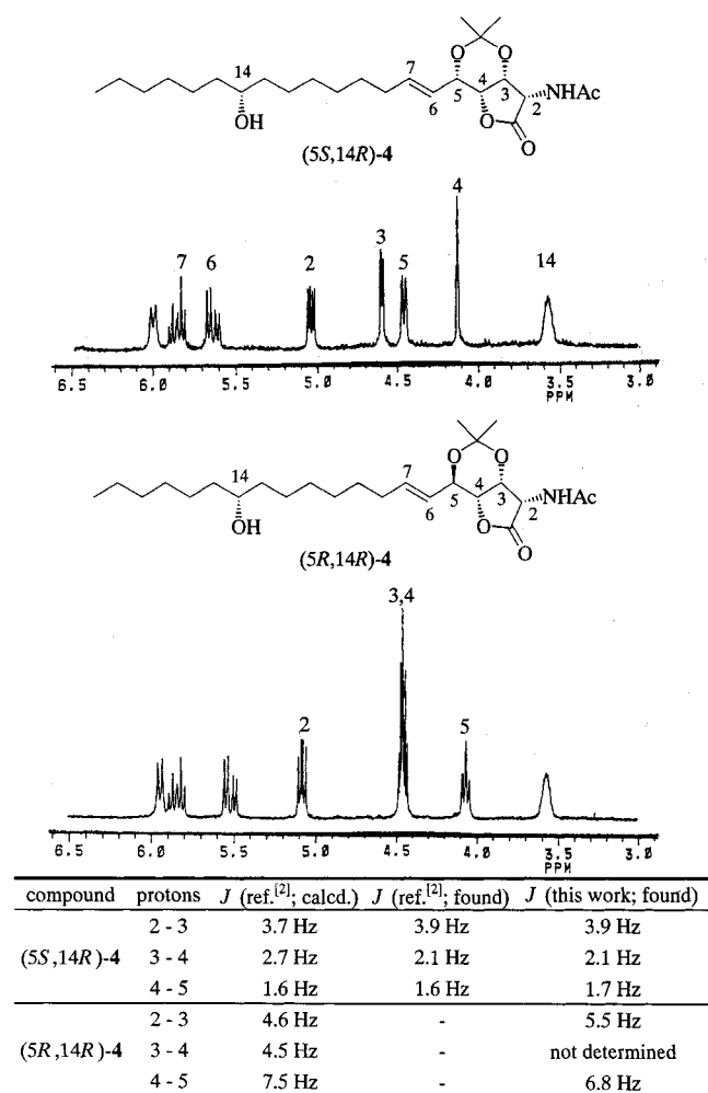
Figure 1. Determination of the stereochemistry of 4 by 300-MHz ^1\text{H} -NMR analysis ( \text{CDCl}_3 )
