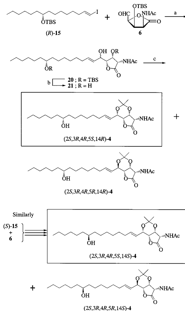
Scheme 4. Synthesis of the four stereoisomers of 4 ; reagents: (a) CrCl 2 (6.0 equiv.), NiCl 2 (0.04 equiv.), DMSO (41%); (b) HF aq., MeCN; (c) Me 2 C(OMe) 2 , TsOH, DMF, chromatog. sepn. [28% of (2 S ,3 R ,4 R ,5 S ,14 R )- 4 based on 20 , 46% of (2 S ,3 R ,4 R ,5 R ,14 R )- 4 based on 20 ]
